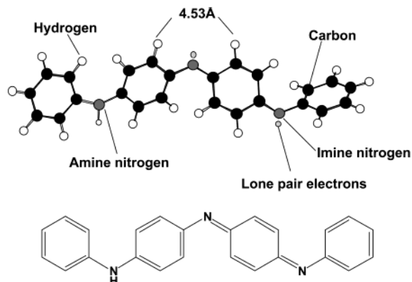
Figure 1. Computer model of the EB tetramer showing the two ortho hydrogens around the imine (above) and the structure of the aniline EB (with the terminal amines removed) (below).
